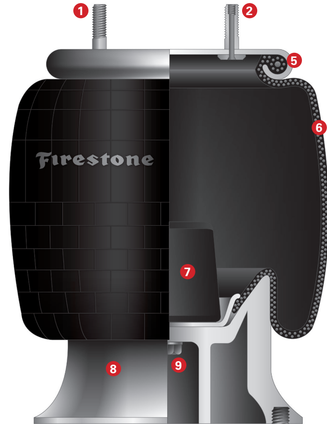
1T Reversible Sleeve Example
